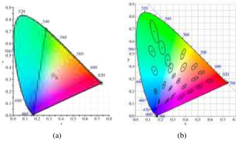
Figure 2.30 CIE chromaticity diagram, showing the pure single-wavelength spectral colors along the perimeter and the white point at E, plotted along their corresponding (x, y) values. (a) the red, green, and blue primaries do not span the complete gamut, so that negative amounts of red need to be added to span the blue–green range; (b) the MacAdam ellipses show color regions of equal discriminability, and form the basis of the Lab perceptual color space.
