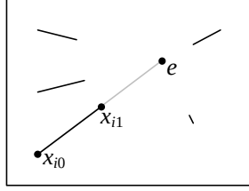
Figure 11.12 Pure translational camera motion results in visual motion where all the points move towards (or away from) a common focus of expansion (FOE) \mathbf{e} . They therefore satisfy the triple product condition (\mathbf{x}_0, \mathbf{x}_1, \mathbf{e}) = \mathbf{e} \cdot (\mathbf{x}_0 \times \mathbf{x}_1) = 0 .
