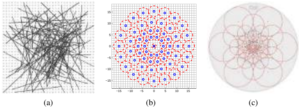
Figure 7.19 Binary bit-string feature descriptors: (a) the BRIEF descriptor compares 128 pairs of pixel values (denoted by line segments) and stores the comparison results in a 128-bit vector (Calonder, Lepetit et al. 2010) © 2010 Springer; (b) BRISK sampling pattern and Gaussian blur radii; (Leutenegger, Chli, and Siegwart 2011) © 2011 IEEE; (c) FREAK retinal sampling pattern (Alahi, Ortiz, and Vanderghenst 2012) © 2012 IEEE.
