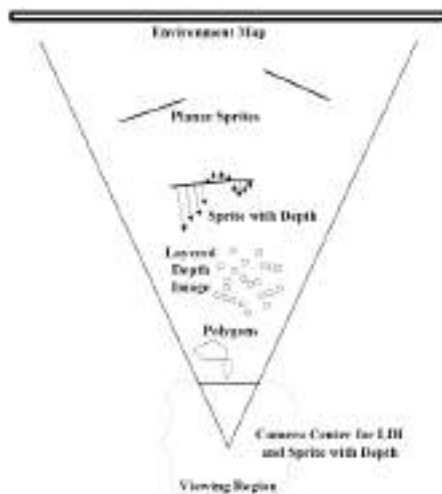
Figure 14.5 A variety of image-based rendering primitives, which can be used depending on the distance between the camera and the object of interest (Shade, Gortler et al. 1998) © 1998 ACM. Closer objects may require more detailed polygonal representations, while mid-level objects can use a layered depth image (LDI), and far-away objects can use sprites (potentially with depth) and environment maps.
