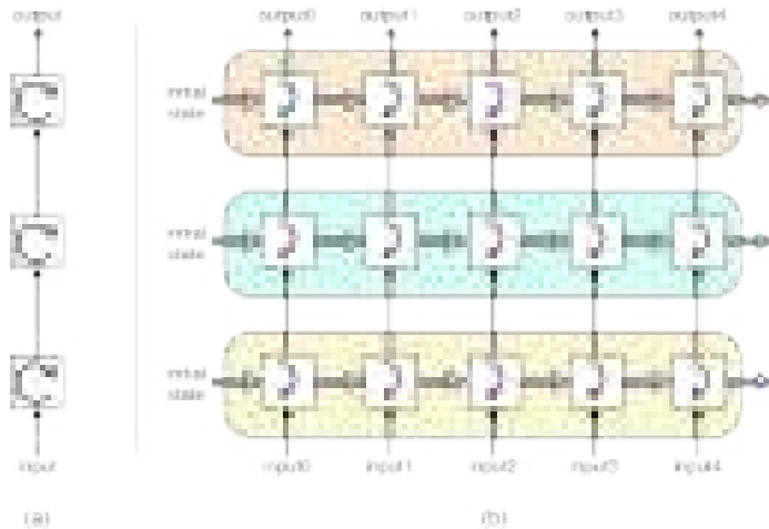
Figure 5.55 A deep recurrent neural network (RNN) uses multiple stages to process sequential data, with the output of one stage feeding the input of the next © Glassner (2018) . Each stage maintains its own state and backpropagates its own gradients, although weights are shared between all stages. Column (a) shows a more compact rolled-up diagram, while column (b) shows the corresponding unrolled version.
