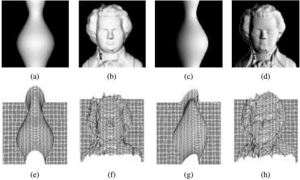
Figure 13.2 Synthetic shape from shading (Zhang, Tsai et al. 1999) © 1999 IEEE: shaded images, (a–b) with light from in front (0, 0, 1) and (c–d) with light from the front right (1, 0, 1); (e–f) corresponding shape from shading reconstructions using the technique of Tsai and Shah (1994).
