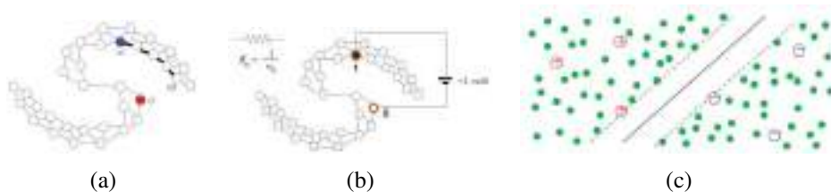
Figure 5.22 Examples of semi-supervised learning (Zhu and Goldberg 2009) © 2009 Morgan & Claypool: (a) two labeled samples and a graph connecting all of the samples; (b) solving binary labeling with harmonic functions, interpreted as a resistive electrical network; (c) using semi-supervised support vector machine (S3VM).
