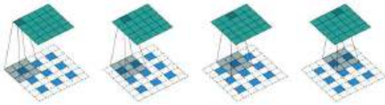
Figure 5.36 Transposed convolution (© Dumoulin and Visin (2016)) can be used to upsample (increase the size of) an image. Before applying the convolution operator, (s \oslash 1) extra rows and columns of zeros are inserted between the input samples, where s is the upsampling stride.
