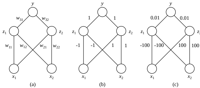
Figure 5.62 Simple two hidden unit network with a ReLU activation function and no bias parameters for regressing the function y = |x_1 + 1.1x_2| : (a) can you guess a set of weights that would fit this function?; (b) a reasonable set of starting weights; (c) a poorly scaled set of weights.
