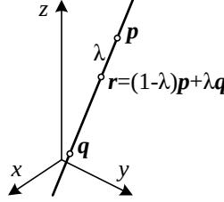
Figure 2.3 3D line equation, \mathbf{r} = (1 \oslash \lambda)\mathbf{p} + \lambda\mathbf{q} .
