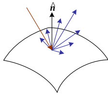
2. Image formation
