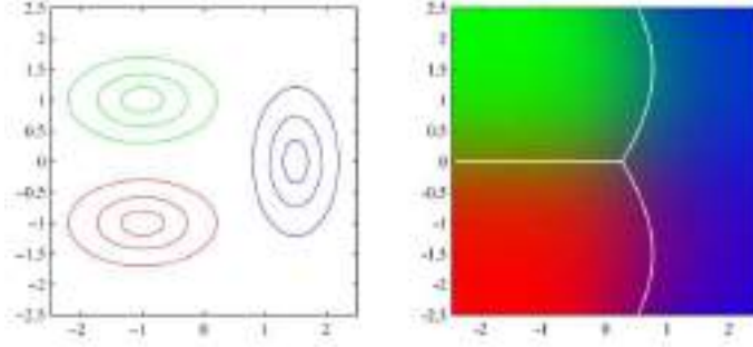
Figure 5.9 Quadratic discriminant analysis (Bishop 2006) © 2006 Springer. When the class covariances \Sigma_k are different, the decision surfaces between Gaussian distributions become quadratic surfaces.
