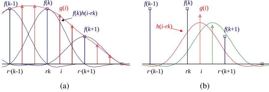
Figure 3.26 Signal interpolation, g(i) = \sum_k f(k)h(i \oslash rk) : (a) weighted summation of input values; (b) polyphase filter interpretation.
