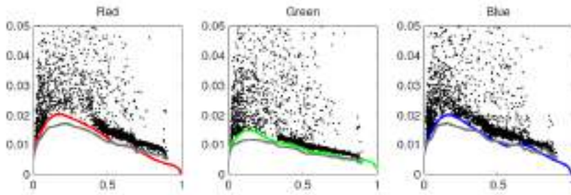
Figure 10.4 Noise level function estimates obtained from a single color photograph (Liu, Szeliski et al. 2008) © 2008 IEEE. The colored curves are the estimated NLF fit as the probabilistic lower envelope of the measured deviations between the noisy piecewise-smooth images. The ground truth NLFs obtained by averaging 29 images are shown in gray.
