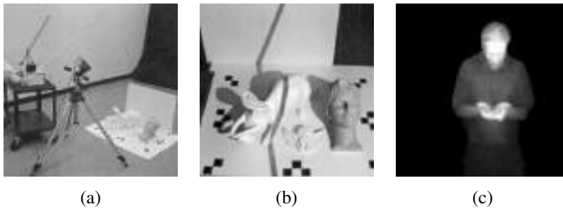
Figure 13.8 Shape scanning using cast shadows ( Bouguet and Perona 1999 ) © 1999 Springer: (a) camera setup with a point light source (a desk lamp without its reflector), a hand-held stick casting a shadow, and (b) the objects being scanned in front of two planar backgrounds. (c) Real-time depth map using a pulsed illumination system ( Iddan and Yahav 2001 ) © 2001 SPIE.
