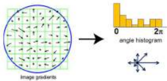
Figure 7.12 A dominant orientation estimate can be computed by creating a histogram of all the gradient orientations (weighted by their magnitudes or after thresholding out small gradients) and then finding the significant peaks in this distribution (Lowe 2004) © 2004 Springer.
