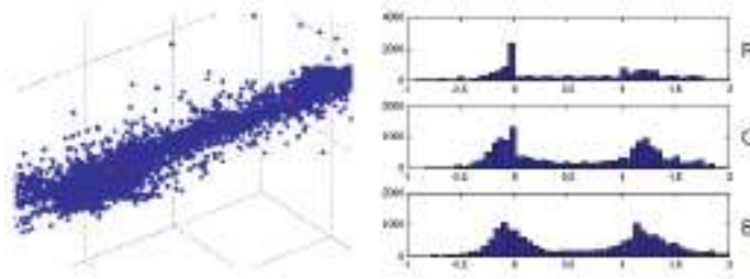
Figure 10.37 Two-color model computed from a collection of local 5 \times 5 neighborhoods (Bennett, Uyttendaele et al. 2006) © 2006 Springer. After two-means clustering and reprojec-tion along the line joining the two dominant colors (red dots), the majority of the pixels fall near the fitted line. The distribution along the line, projected along the RGB axes, is peaked at 0 and 1, the two dominant colors.
