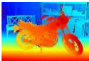
12. Depth estimation
