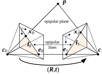
Figure 11.11 Epipolar geometry: The vectors \mathbf{t} = \mathbf{c}_1 \mathcal{O} \mathbf{c}_0 , \mathbf{p} \mathcal{O} \mathbf{c}_0 and \mathbf{p} \mathcal{O} \mathbf{c}_1 are co-planar and define the basic epipolar constraint expressed in terms of the pixel measurements \mathbf{x}_0 and \mathbf{x}_1 .
