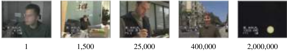
Figure 10.11 Relative brightness of different scenes, ranging from 1 inside a dark room lit by a monitor to 2,000,000 looking at the Sun. Photos courtesy of Paul Debevec.
